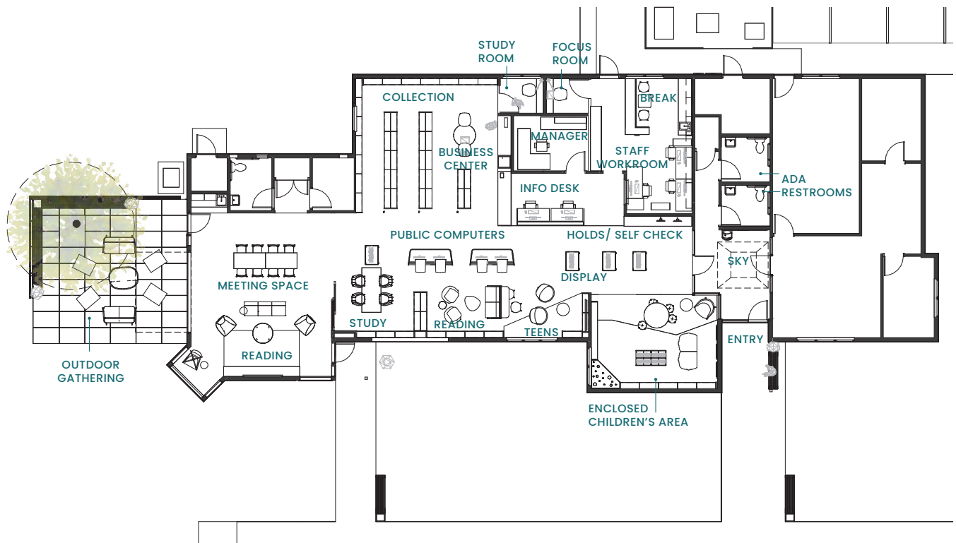
Proposed Floorplan
