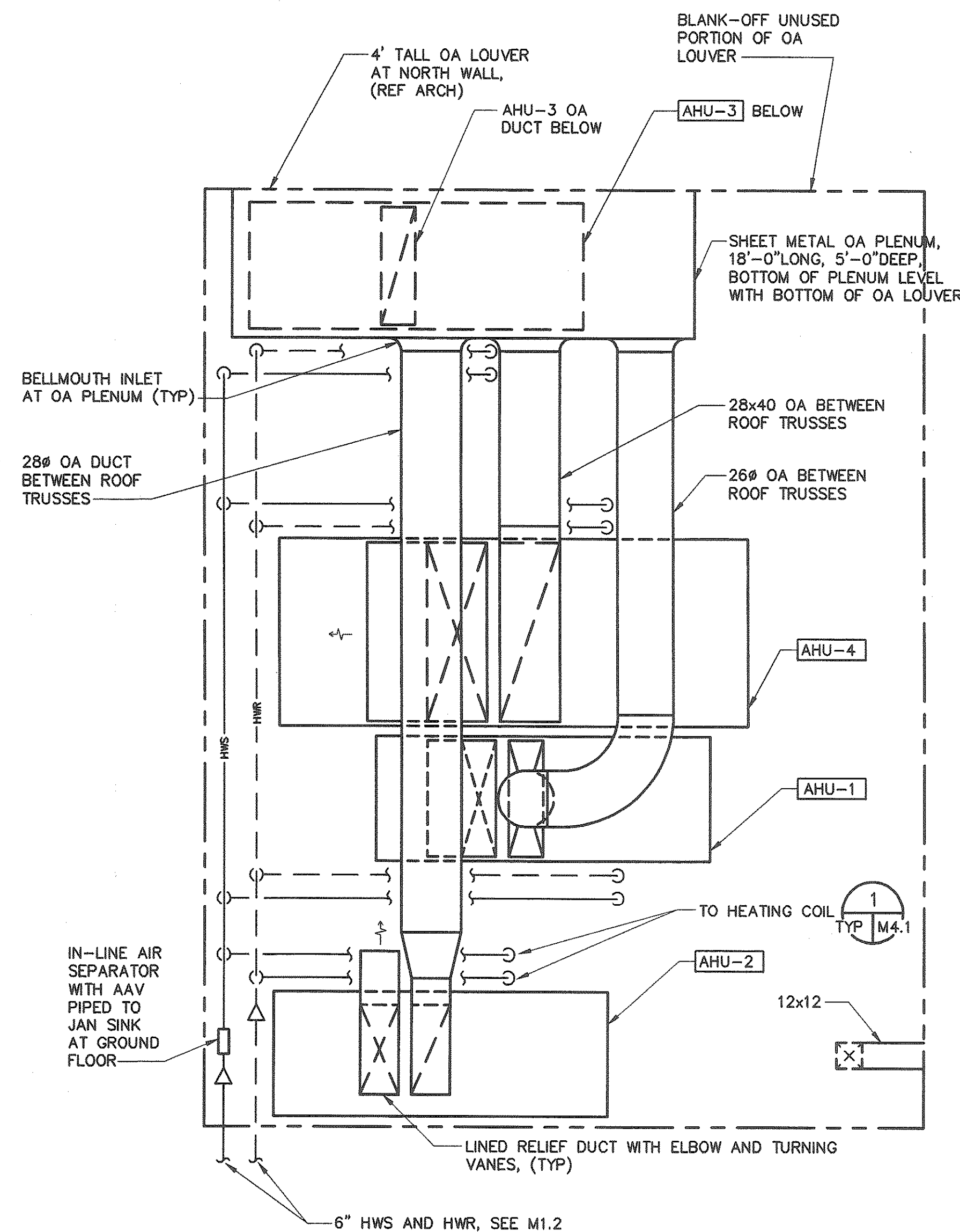
MEZZANINE MECHANICAL ROOM UPPER LEVEL ENLARGED PLAN (2) SCALE: 1/4" = 1'-0"
