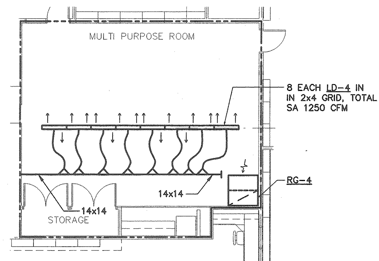
MULTI PURPOSE ROOM HVAC PARTIAL PLAN (3) SCALE: 1/8" = 1'-0"
