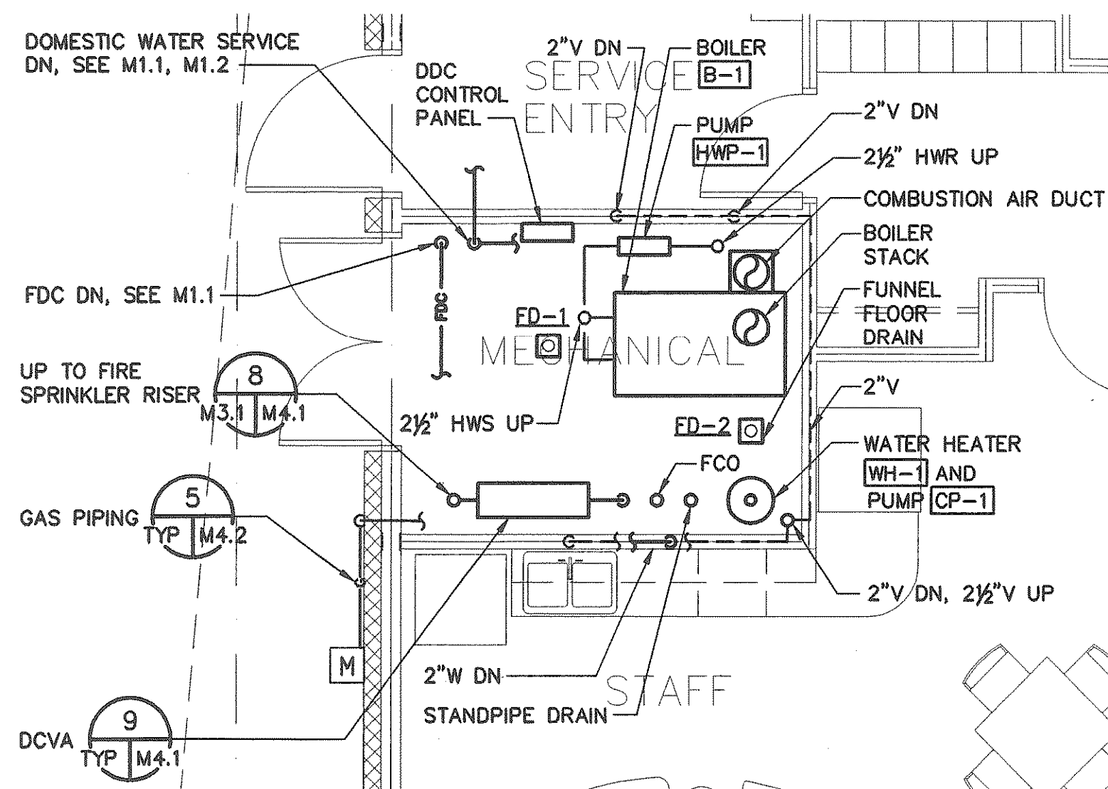
MECHANICAL ROOM ENLARGED PLAN (4) SCALE: 1/4" = 1'-0"
