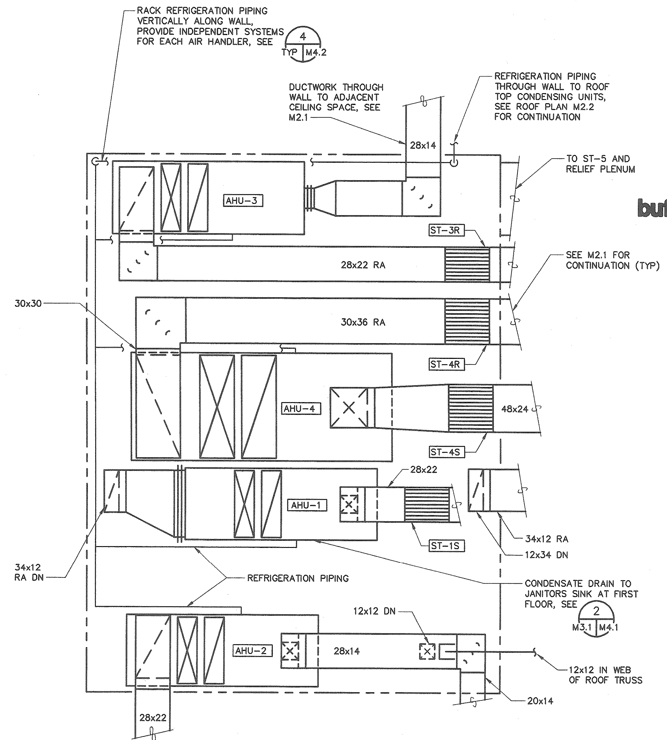
MEZZANINE MECHANICAL ROOM LOWER LEVEL ENLARGED PLAN (1) SCALE: 1/4" = 1'-0"
